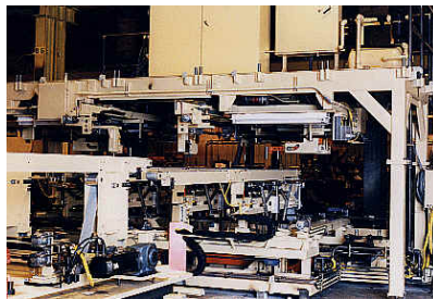
High Speed Overhead Centering Conveyor
